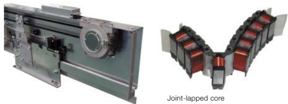
Joint-lapped core
